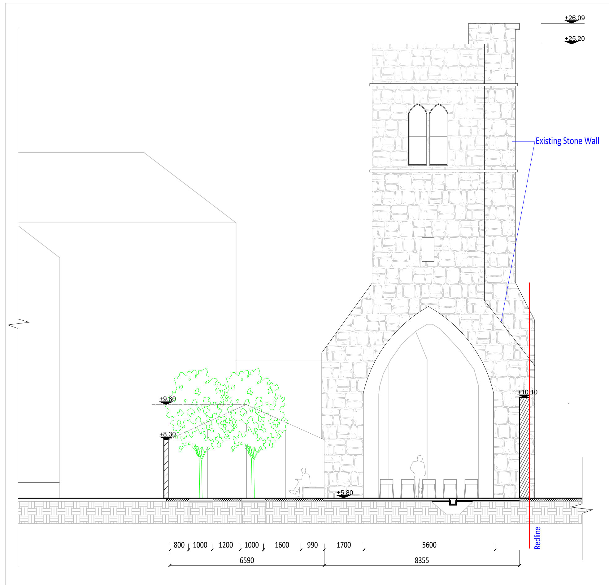
SECTION C-C 1:100
